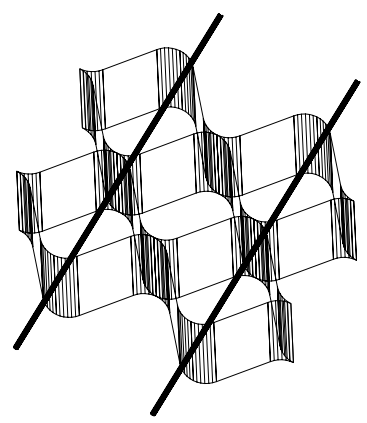
TYPICAL TENDON DETAIL
